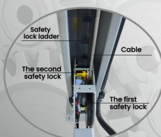
Double-safety locks
